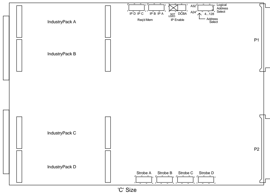
Figure 3. Hardware Configurable Controls
