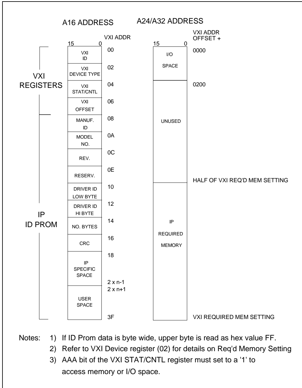
Figure 2. Memory Organization
