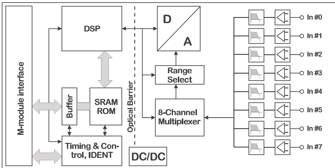
Figure 3 M393 Block Diagram
