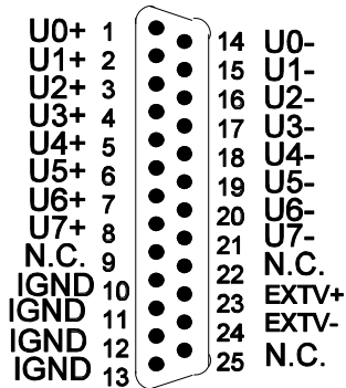
Figure 2 Front view 25 pole D-sub
