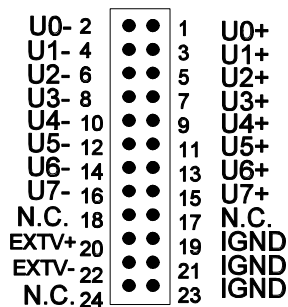
Figure 1 Top view 24 pole female header. Not available on M393/R0.x
