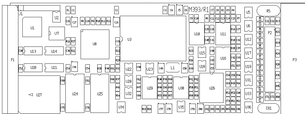
Figure 7 M393 Component Image
