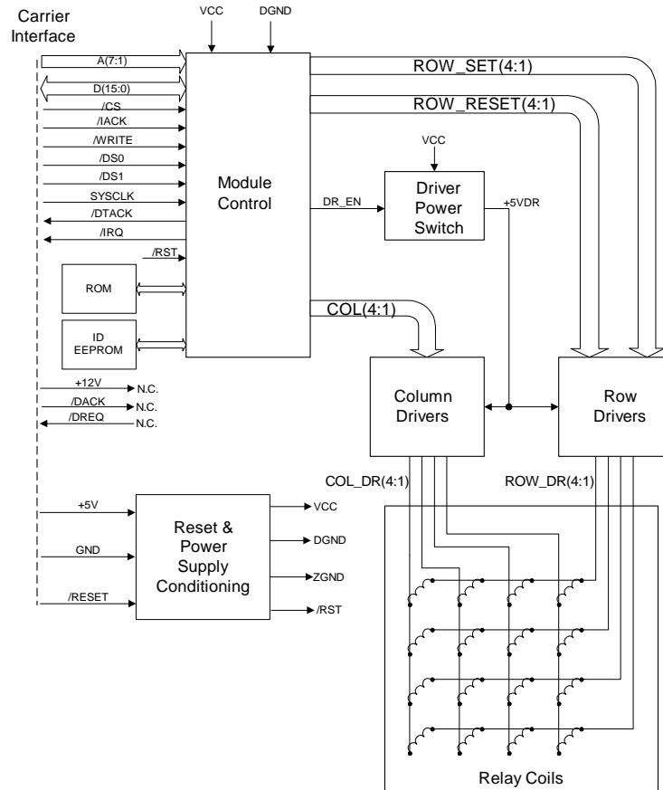
Figure 2. M218 Functional Block Diagram
