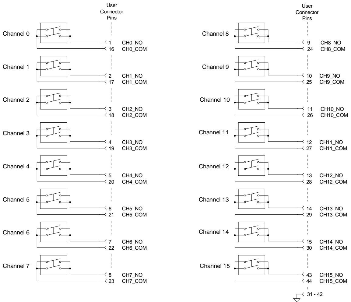
Figure 3. M218 Switching Schematic
