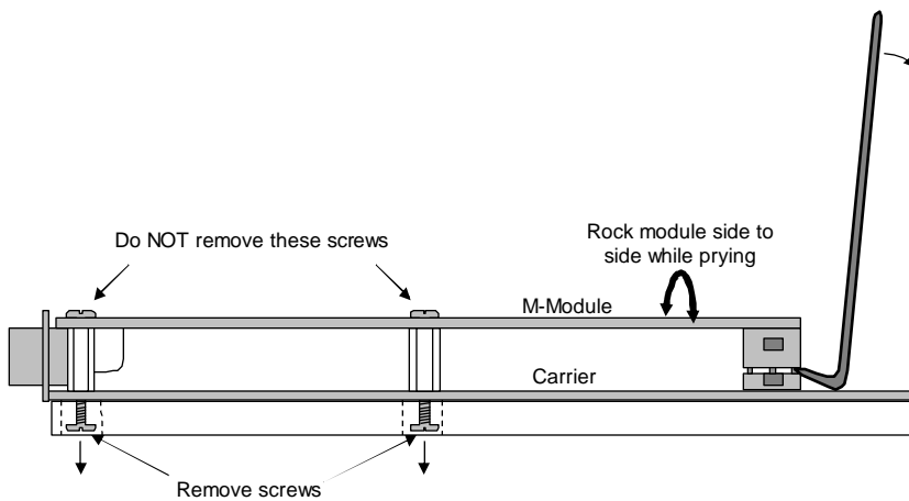
Figure 4. M-Module Removal
